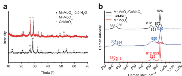
Figure 1 | Phase analysis. (a) XRD patterns of backbone MnMoO 4 nanowires (black line) and hierarchical MnMoO 4 /CoMoO 4 heterostructured nanowires (red line). (b) Raman spectra of hierarchical MnMoO 4 /CoMoO 4 heterostructured nanowires, pure CoMoO 4 nanorods and backbone MnMoO 4 nanowires.
