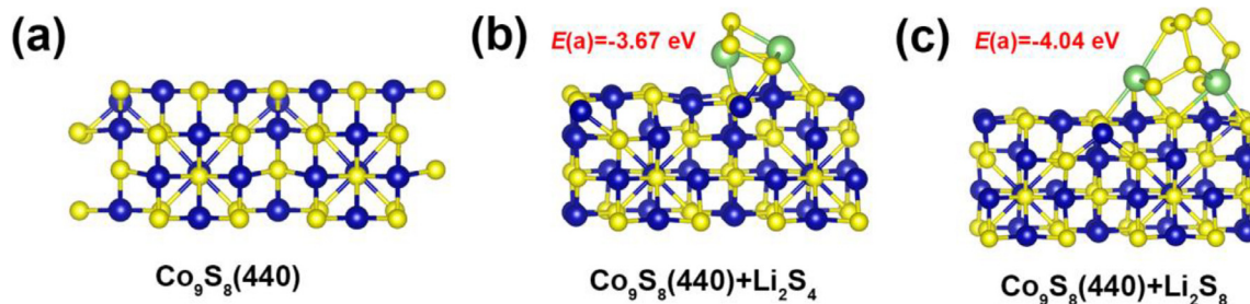
Fig. 4. (a) The optimized structures of the \text{Co}_9\text{S}_8(440) surface and its adsorption models of binding with (b) \text{Li}_2\text{S}_4 and (c) \text{Li}_2\text{S}_8 , respectively.
