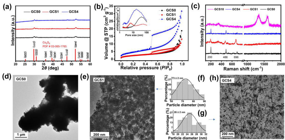
Fig. 2. (a) PXRD patterns of GCS0, GCS1 and GCS4 and the indexed PDF card. (b) \text{N}_2 adsorption/desorption isotherms of GCS0, GCS1 and GCS4, inset is the pore distribution curve of them. (c) Raman spectra of GCS0, GCS1, GCS4 and GCS10. TEM images of (d) GCS0, (e) GCS1 and (h) GCS4 and corresponding size distribution diagrams of (f) GCS1 and (g) GCS4.
