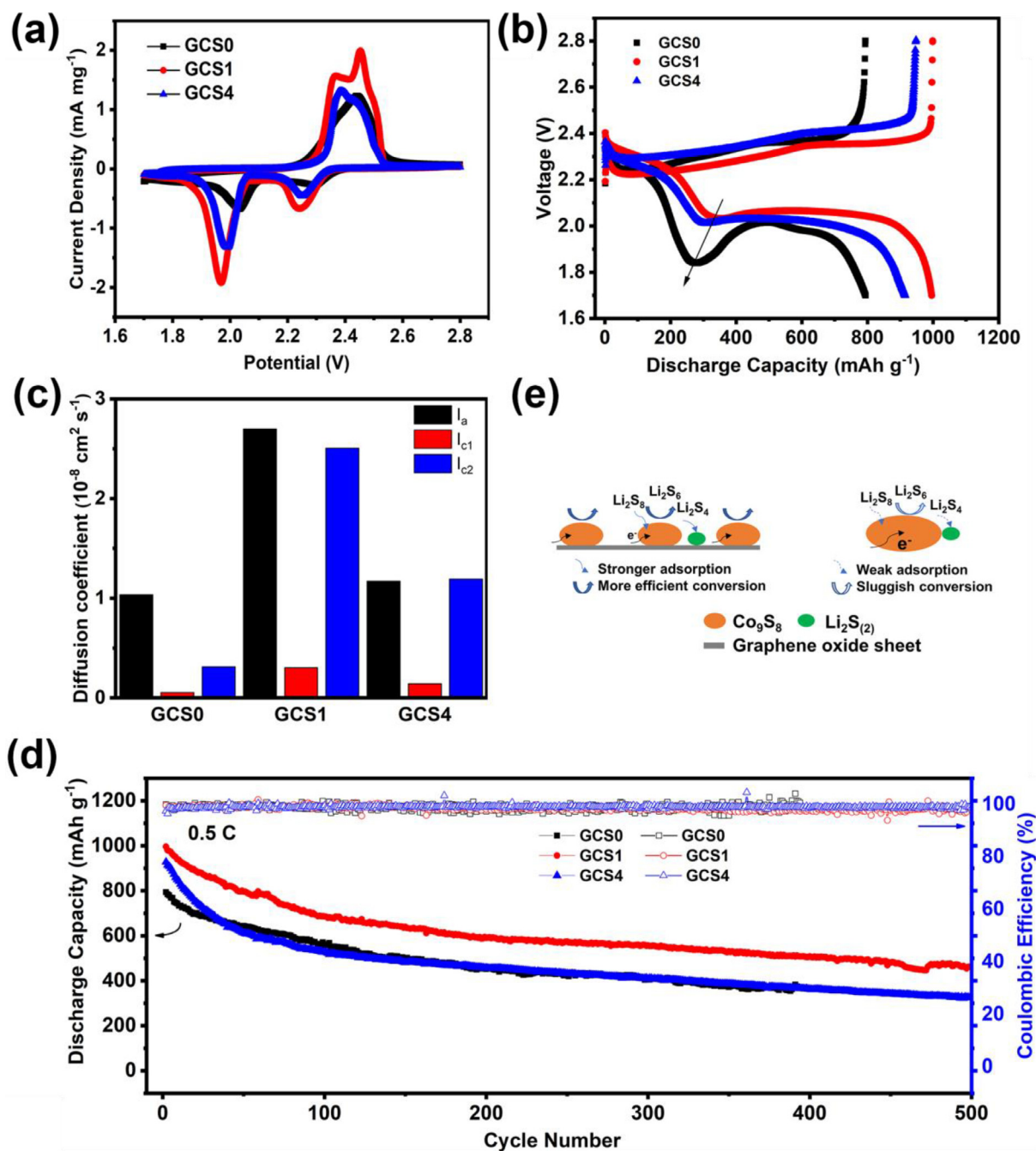
Fig. 5. (a) CV curves scanned at 0.1 \text{ mV s}^{-1} , (b) Typical charge/discharge voltage curves at 0.5 \text{ C} , (c) Calculated lithium ion diffusion coefficients from three redox peaks of the corresponding CV curves ( I_a , I_{c1} and I_{c2} correspond to the anodic peak, first cathodic peak and second cathodic peak, respectively) and (d) Long-term cycling curves at 0.5 \text{ C} of the Li-S batteries enabled by GCS0-S, GCS1-S and GCS4-S composites. (e) Comparison of different electrochemical mechanisms of GCS1 (left) and GCS0 (right) in Li-S batteries.
